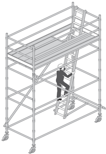
Figure 5 Mobile scaffold
